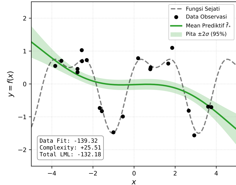
Kasus A: Underfitting / Over-smooth ( l = 4.50, \sigma_n = 0.20 )
