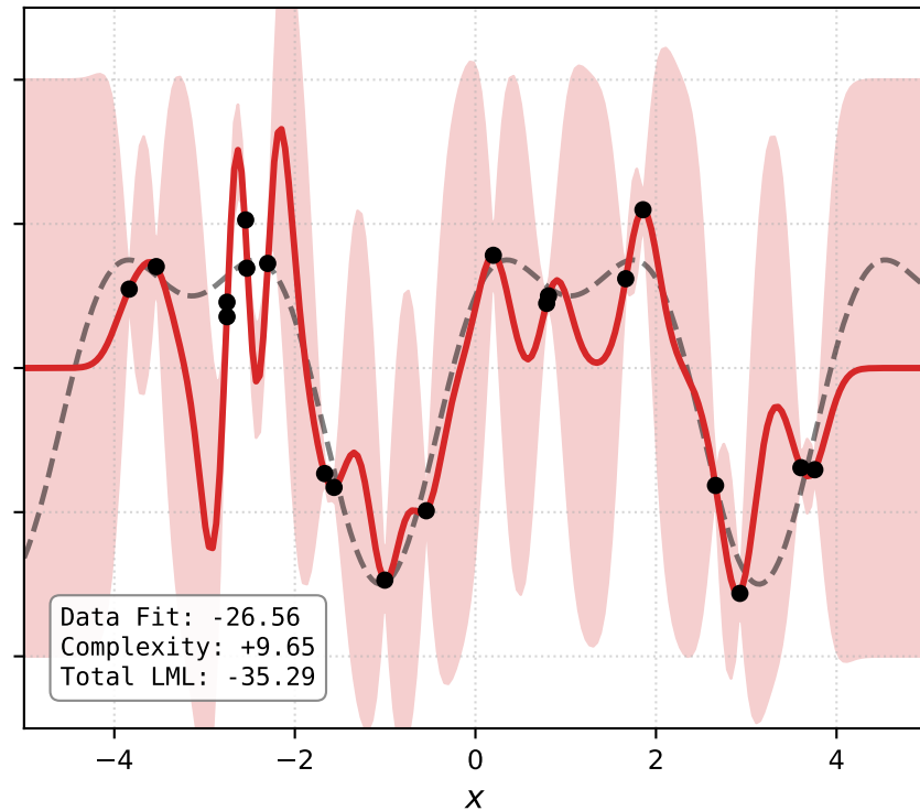
Kasus C: Overfitting / Over-complex ( l = 0.18, \sigma_n = 0.03 )
